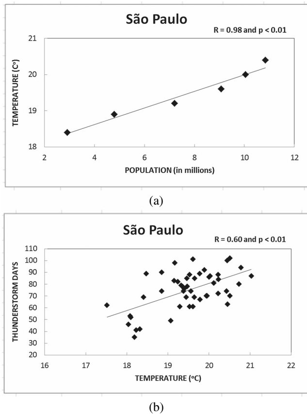
Figure 6. Linear regression between (a) the average annual surface temperature versus annual population for some specific years (see text for details) and (b) average annual number of thunderstorm days versus average annual surface temperature for São Paulo after 1951.
