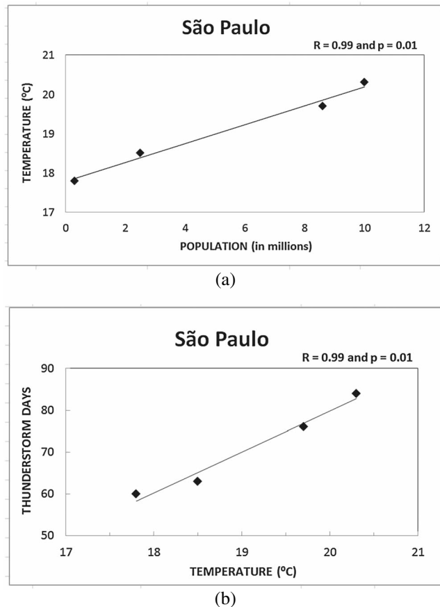
Figure 9. Linear regression between (a) the average temperature versus average annual population and (b) the average annual number of thunderstorm days versus average temperature for the values in Table 1.
