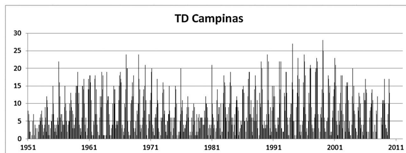
Figure 10. Time series of monthly thunderstorm day for Campinas after 1951.
